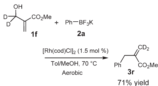
Scheme 1. Regioselectivity of the addition.
